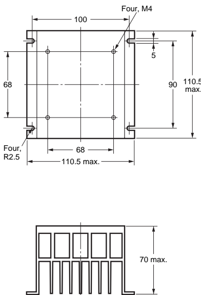
Mounting Holes
