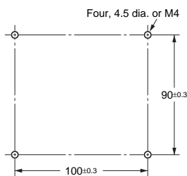
Mounting Holes
