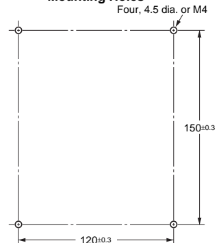
Mounting Holes
