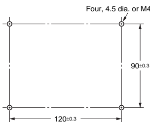
Mounting Holes
