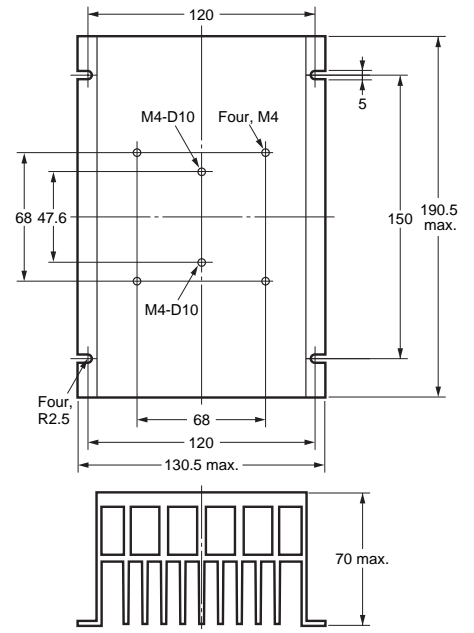
Mounting Holes
