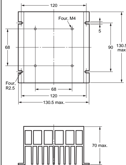
Mounting Holes
