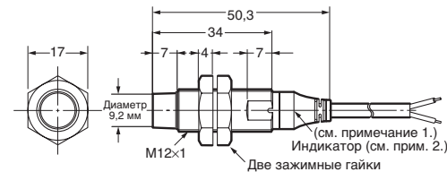
E2A-M12KN08-WP-□□/E2A-S12KN08-WP-□
